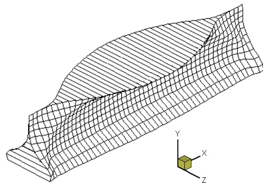
Figure 7. Optimum design of a simply-supported beam subjected to a horizontally-moved vertical load.
