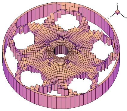
Figure 8. Optimum design of a center-supported wheel subjected to a torque on the rim.
