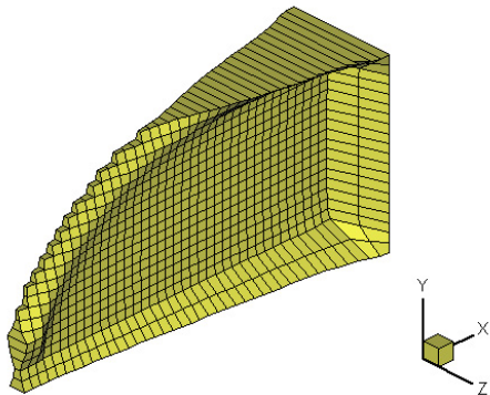
(c) Optimum design after trimming. (the 250 th iteration)
