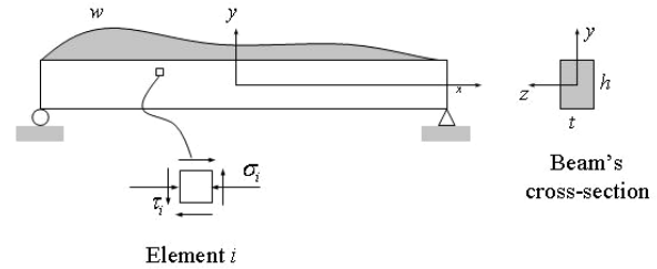
Figure 2. A simply supported beam under distributed load.
