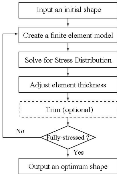
Figure 1. Topology Optimization Procedure.
