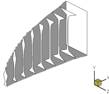
Figure 6. Cross-sections of the final design. (z-scale is magnified three time)
