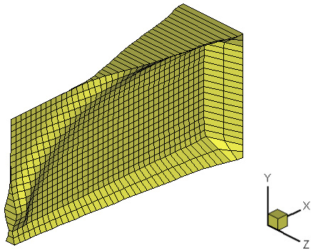
(b) Fully-stressed design. (the 199 th iteration)
